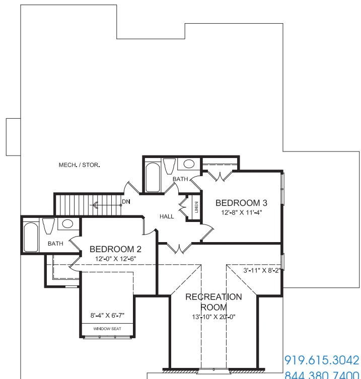
SECOND FLOOR
